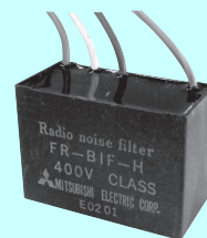
FR-BIF-H
